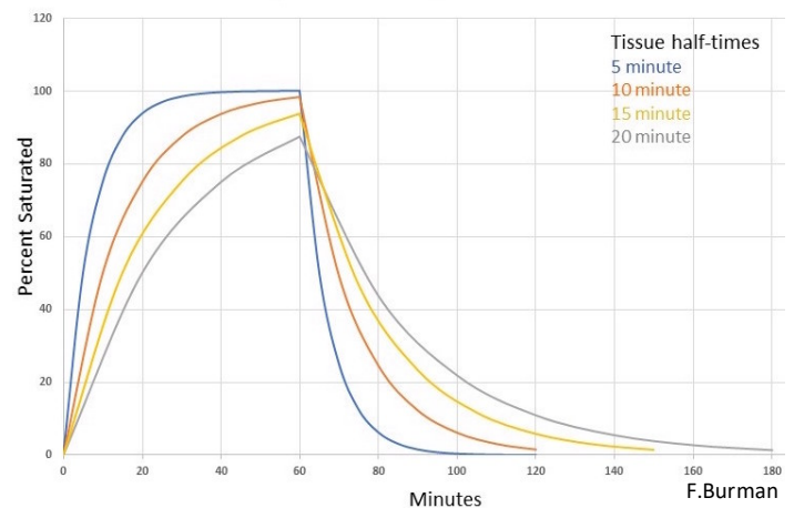
Nitrogen Saturation/Desaturation Curves
